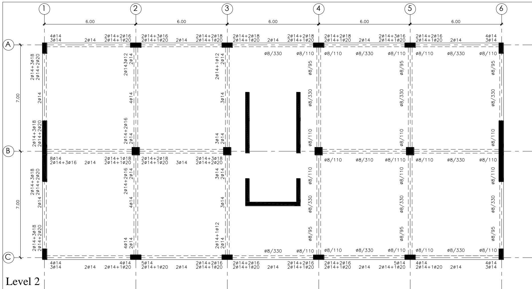
Fig. 3.5.10 Beam framing plan at storey 2
