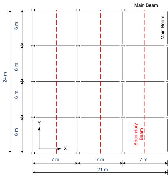
Fig. 5.15.1 Floor plan
